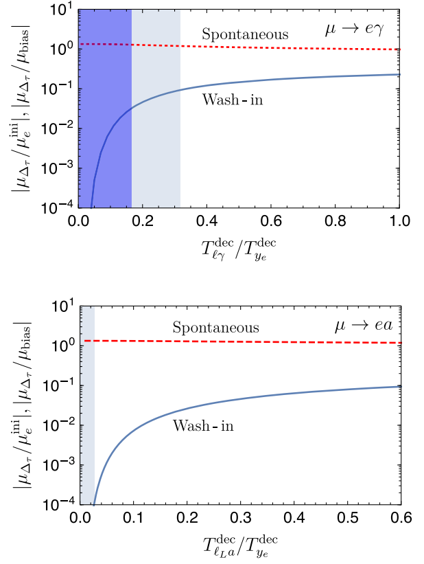
FIG. 1. |\mu_{\Delta_\tau}/\mu_e^{\text{ini}}| for wash-in (blue solid line) and |\mu_{\Delta_\tau}/\mu_{\text{bias}}| for spontaneous (red dashed line) leptoflavorgenesis as functions of T_{\ell\gamma}^{\text{dec}}/T_{y_e}^{\text{dec}} for the LFV process \mu \rightarrow e\gamma (top panel) and T_{\ell La}^{\text{dec}}/T_{y_e}^{\text{dec}} for the LFV process \mu \rightarrow ea (bottom panel). The dark shaded region is excluded by current experimental bounds, while the light shaded region corresponds to the future expected sensitivity.
